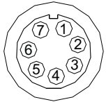
7 pins Binder 712 male connector Solder termination view
