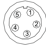
5 pins Binder 712 male connector Solder termination view
